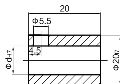
SK19-RH 轴套内径Reducing sleeve d=10,11,12,14,15,16,18mm
