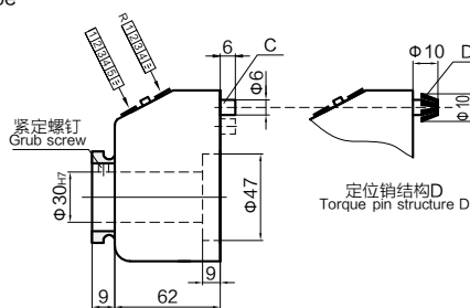
定位销结构C Torque pin structure C
